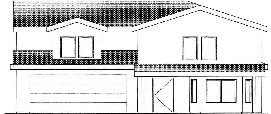
FRONT "A" ELEVATION
