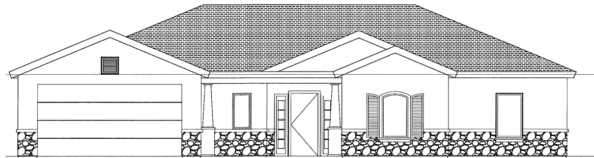
FRONT "C" ELEVATION
