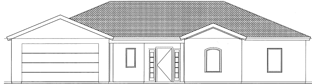
FRONT "A" ELEVATION
